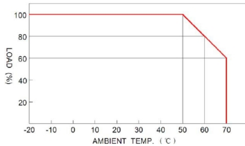
Derating Curve (負荷電力輕減曲線)
