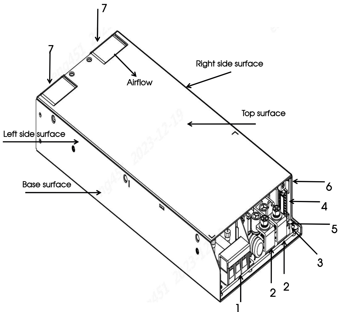
Fig. 1: Appearance information of ZAMF-2000-Bxx Overview description:
